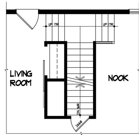
PART. FIRST FLOOR PLAN W/ OPT. LIVING RM. DESK
