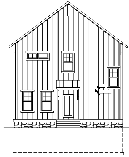
REAR ELEVATION
