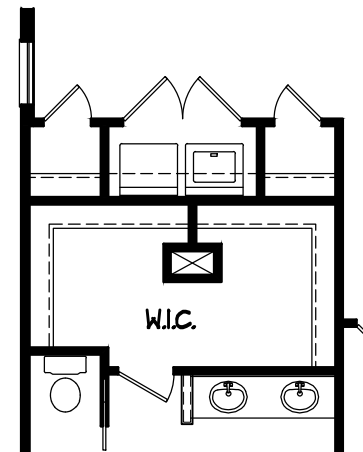
PART. SECOND FLOOR PLAN W/ OPT. LAUNDRY #2
