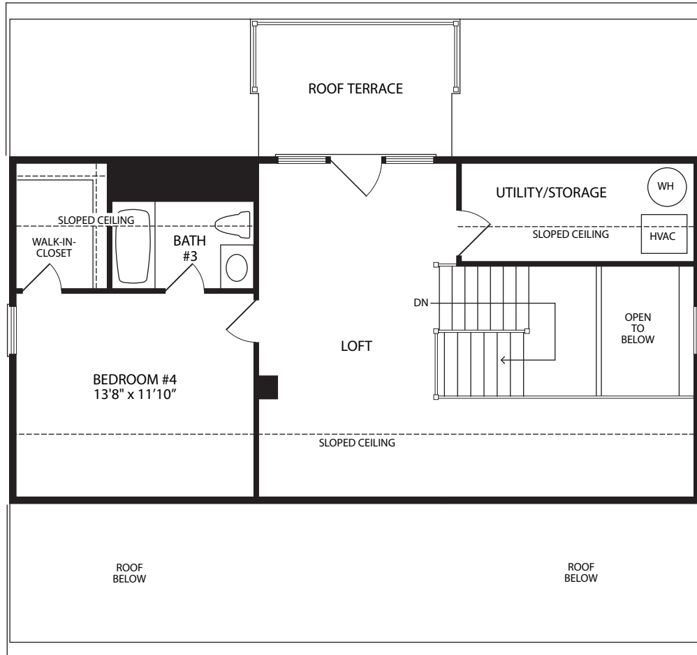
ATTIC FLOOR PLAN LOT 5
