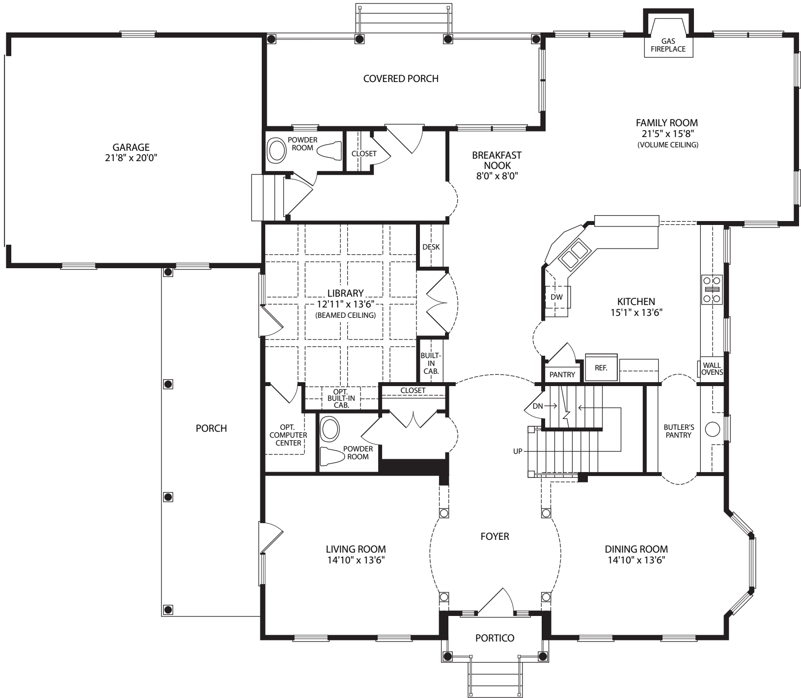
FIRST FLOOR PLAN LOT 1
