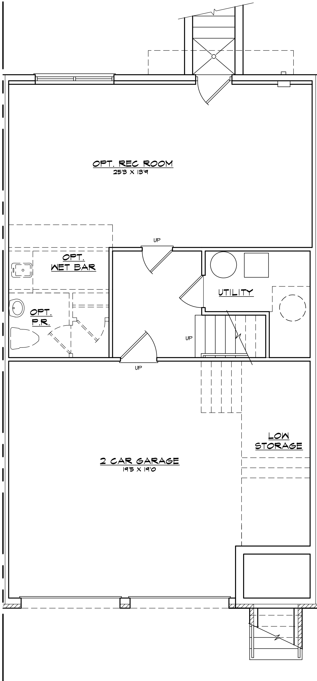
GROUND FLOOR PLAN MODEL B
